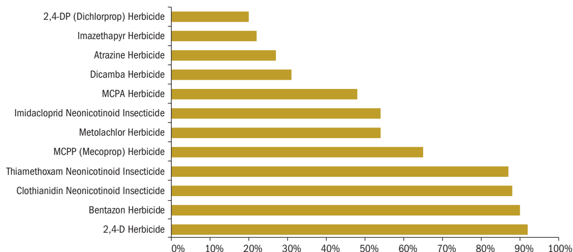
Figure 27: Pesticide Detection Frequencies* in Southern Ontario Agricultural Streams, 2015–2019
