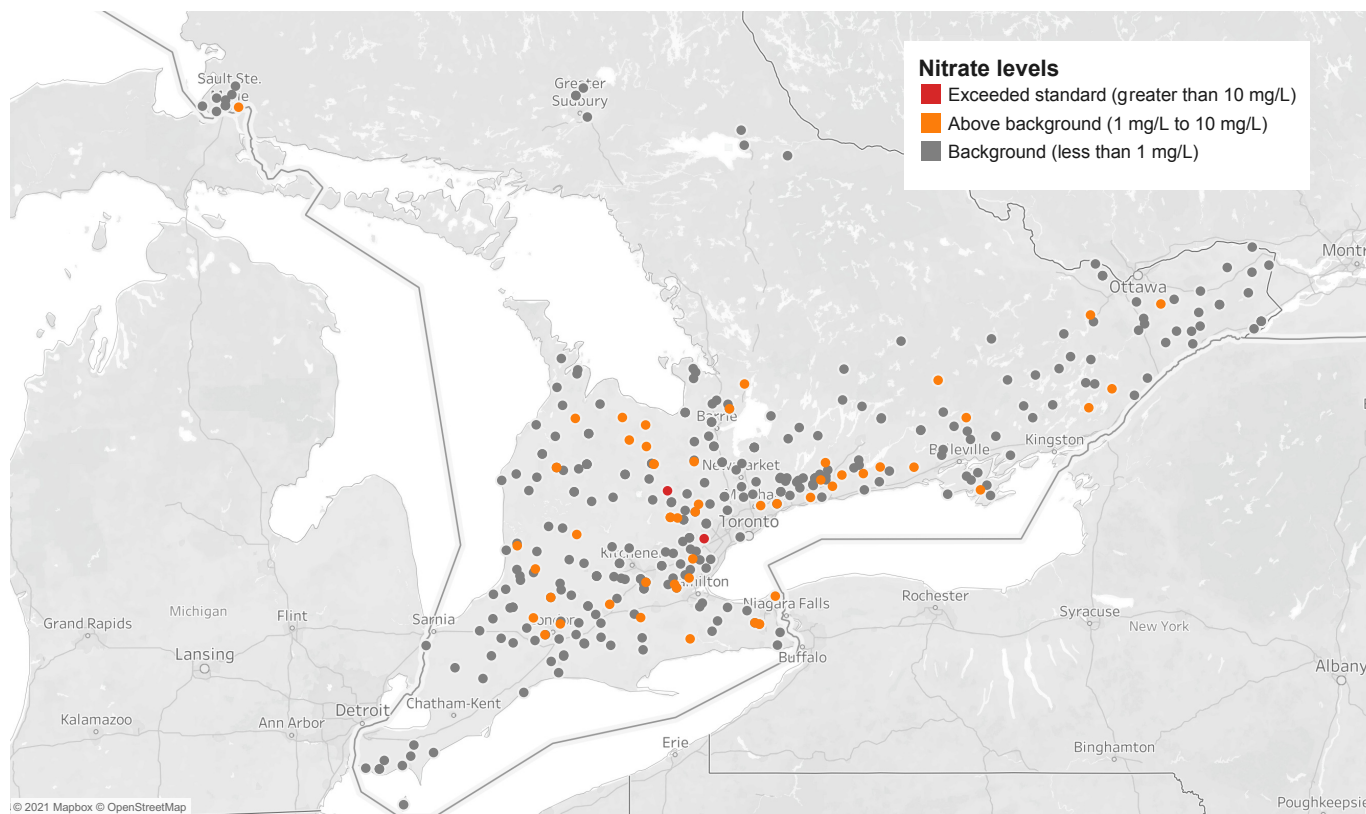
Figure 31: Location and Measurement of Nitrate Levels in Ontario's Monitored Wells,* 2018
