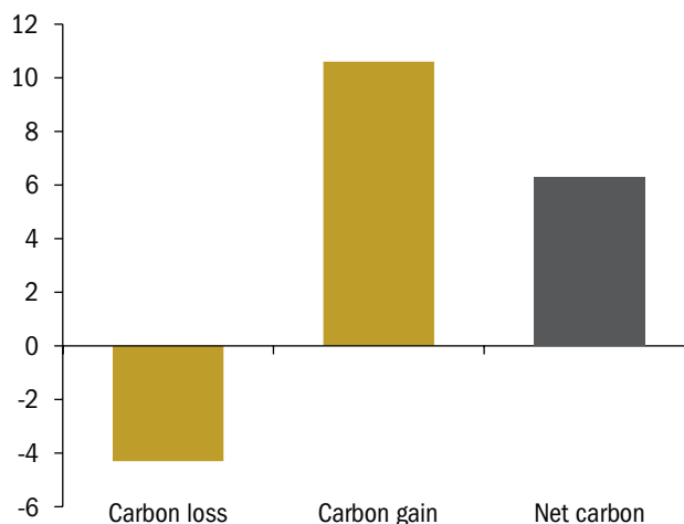
Figure 50: Estimated Average Amount of Net Carbon Stored in Peatlands in Ontario's Far North per Year (million tonnes)
