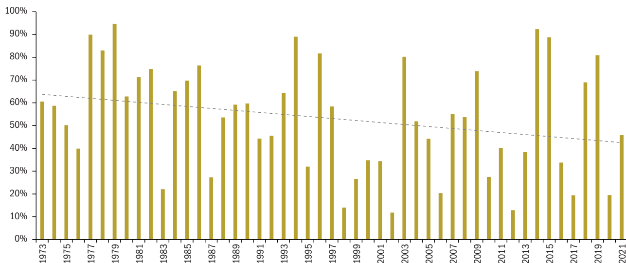
Figure 52: Estimated Annual Maximum Ice Cover (% of Lake Area) in the Great Lakes, * 1973–2021
