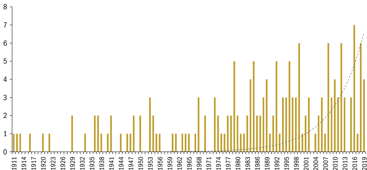
Figure 51: Number of Weather-Related Disasters* in Ontario per Year, 1911–2019
