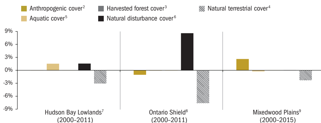
Figure 37: Percentage Changes in Land Cover Composition in Each Ontario Ecozone, 1 2000–2015
