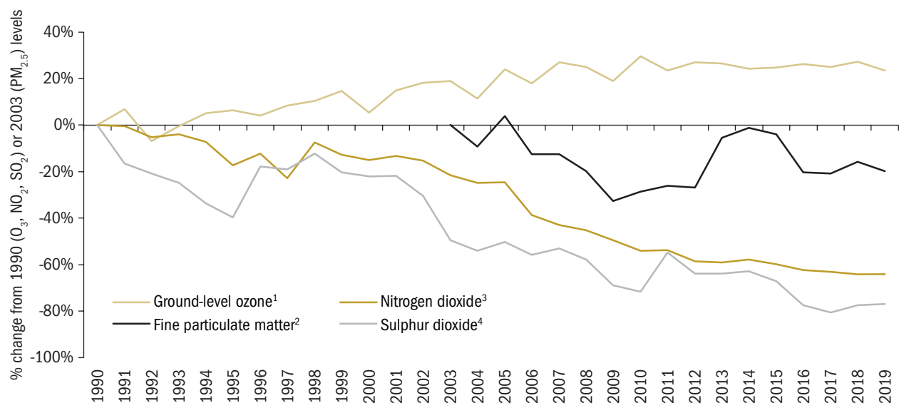
Figure 4: Average Ground-Level Ozone ( O_3 ), Fine Particulate Matter ( PM_{2.5} ), Nitrogen Dioxide ( NO_2 ), and Sulphur Dioxide ( SO_2 ) Concentration Trends at Environment Ministry Air Monitoring Stations, 1990–2019
