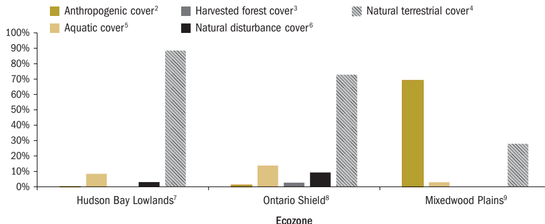
Figure 36: Composition of Each Ontario Ecozone 1 by Land Cover Type
